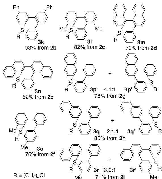
Scheme 2. Products of the arylative ring opening of 2b–i (the structures of which are shown in the Supporting Information).
